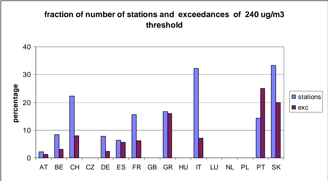
Figure 3.4. Number of stations and number of reported exceedances of the alert threshold (proposed Directive, 240 \mu\text{g}/\text{m}^3 ) expressed as percentage of the number of stations and number of reported exceedances of the information threshold (current Directive, 180 \mu\text{g}/\text{m}^3 ), respectively; Summer 2001; countries reporting no exceedances of the 180 \mu\text{g}/\text{m}^3 threshold are not shown.
