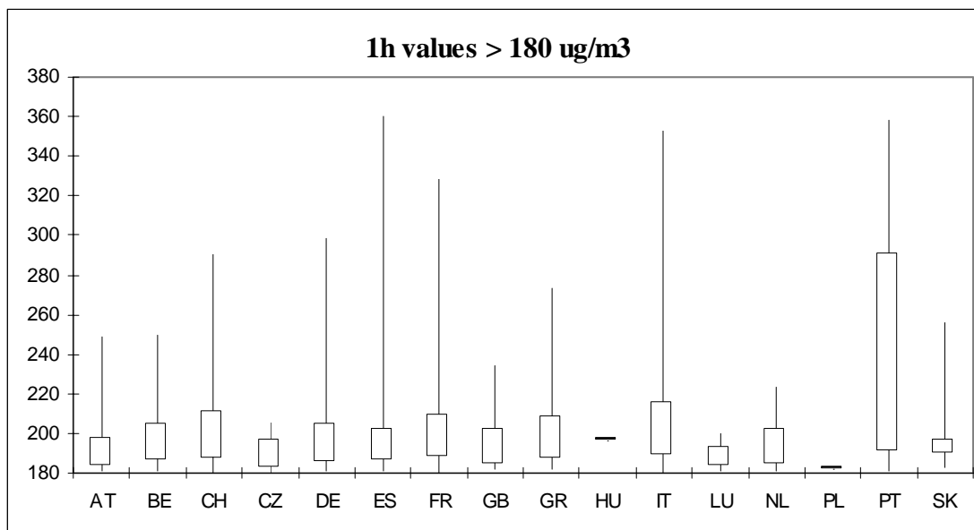
Figure 3.3. Top: Frequency distribution of ozone concentrations in excess of the 180 \mu\text{g}/\text{m}^3 threshold for hourly values (April-August 2001). Frequency distributions are presented as Box-Jenkins plots indicating the minimum, the 25-Percentile, the 75-Percentile and the maximum value. Countries reporting no exceedances are not shown. Bottom: total number of exceedances (#Ex) and number of reporting stations (#St) per country (ISO 3166-1:1997 Alpha-2 code).
