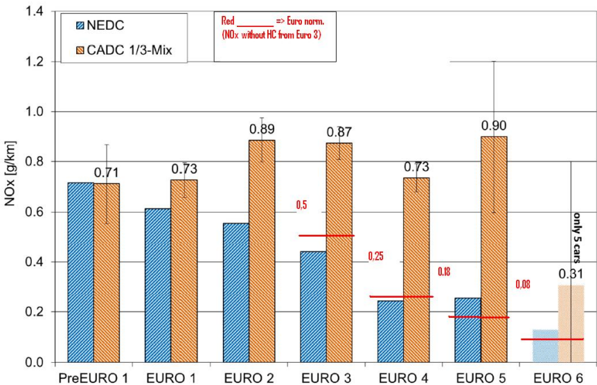
Figure 2: Comparison of the NO x emission factors based on NEDC, CADC and Euro standards (diesel cars) 4
