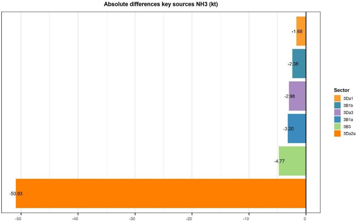
Figure 2 9 Absolute NH 3 emission differences from 1990 to 2022 for all key sectors.
