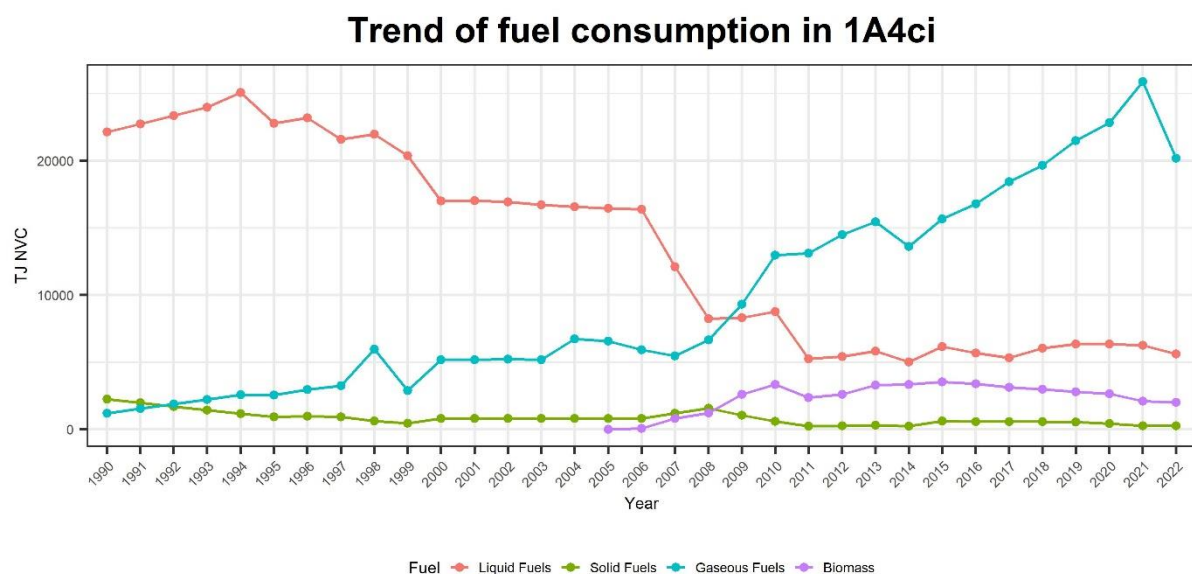
Figure 3 6 Trend of fuel consumption in the agricultural sector
