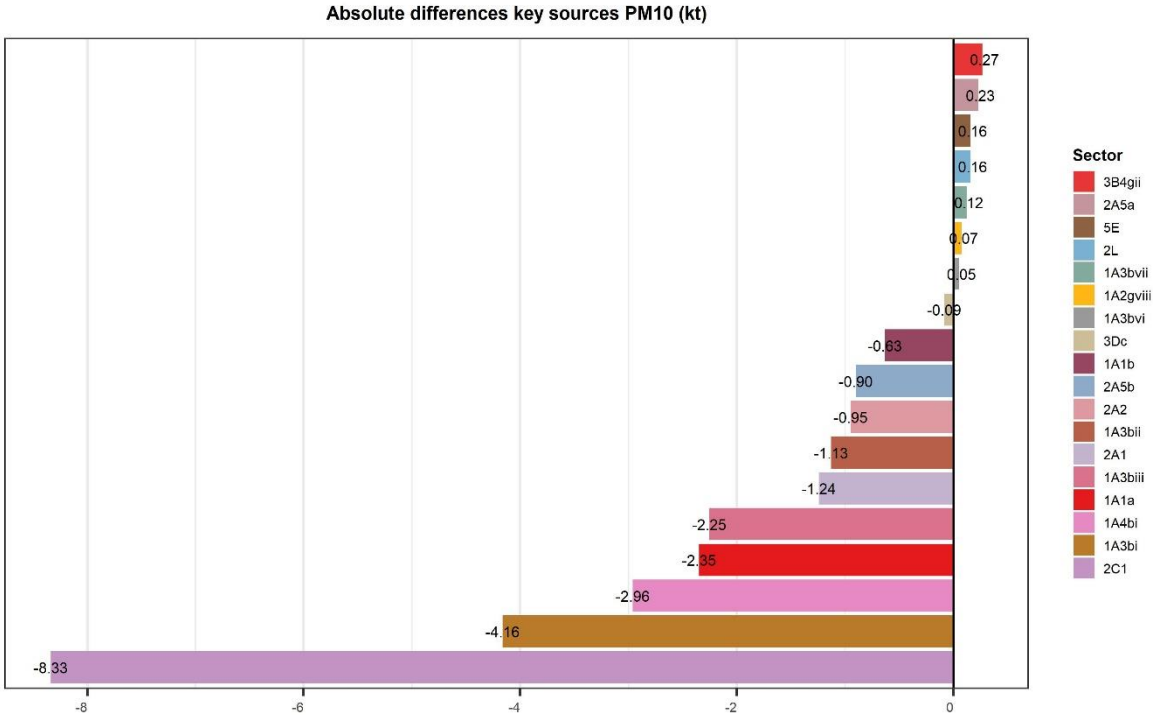
Figure 2 12 Trends in PM 10 emissions for the key sectors
