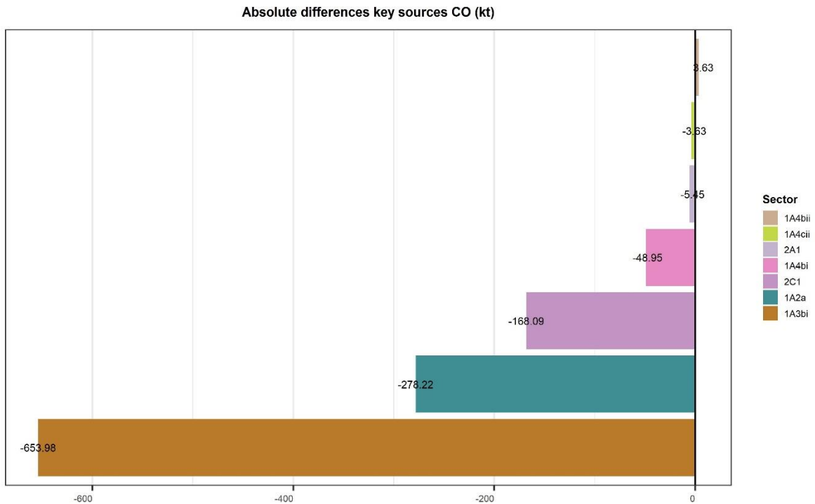
Figure 2 10 Trends in CO emissions for the key sectors
