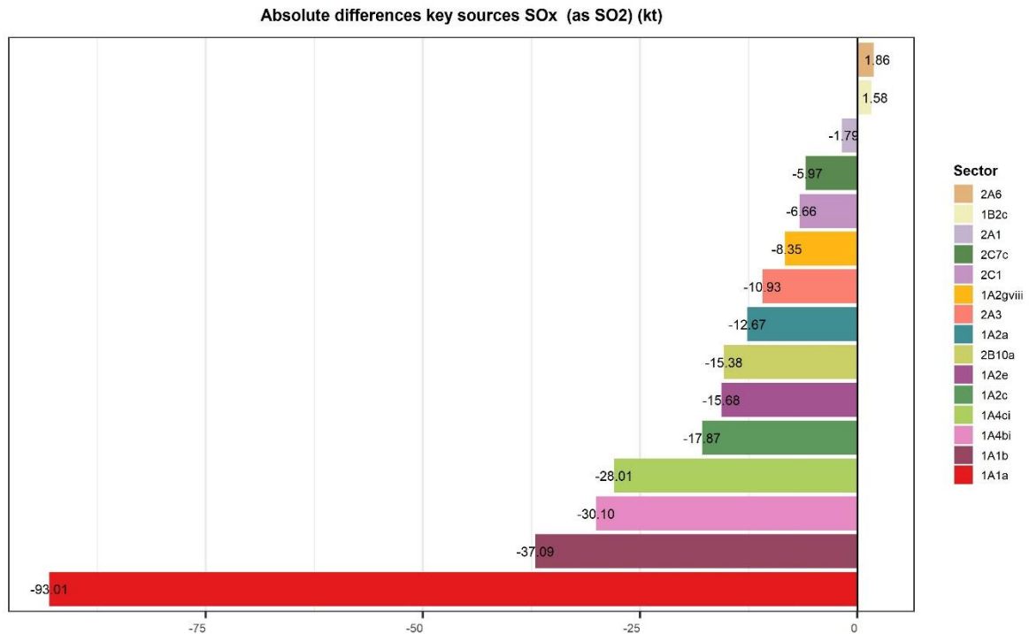
Figure 2 6 Trends in SO x emissions for the key sectors
