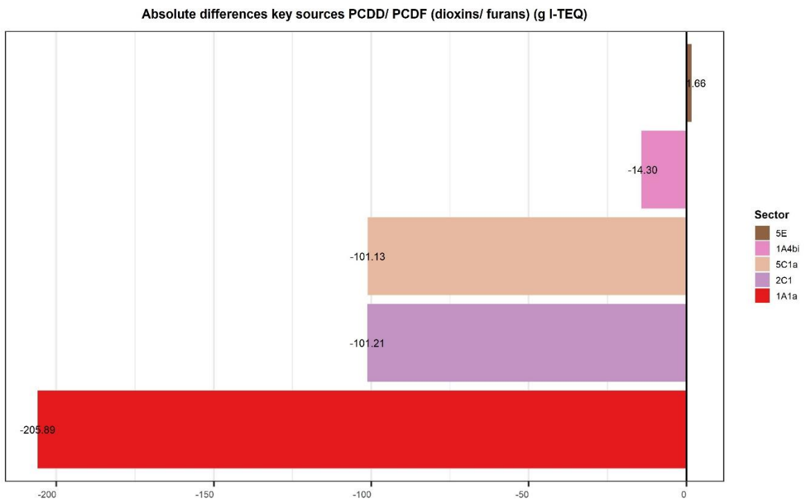
Figure 2 16 Trends in PCDD–PCDF emissions for the key sectors
