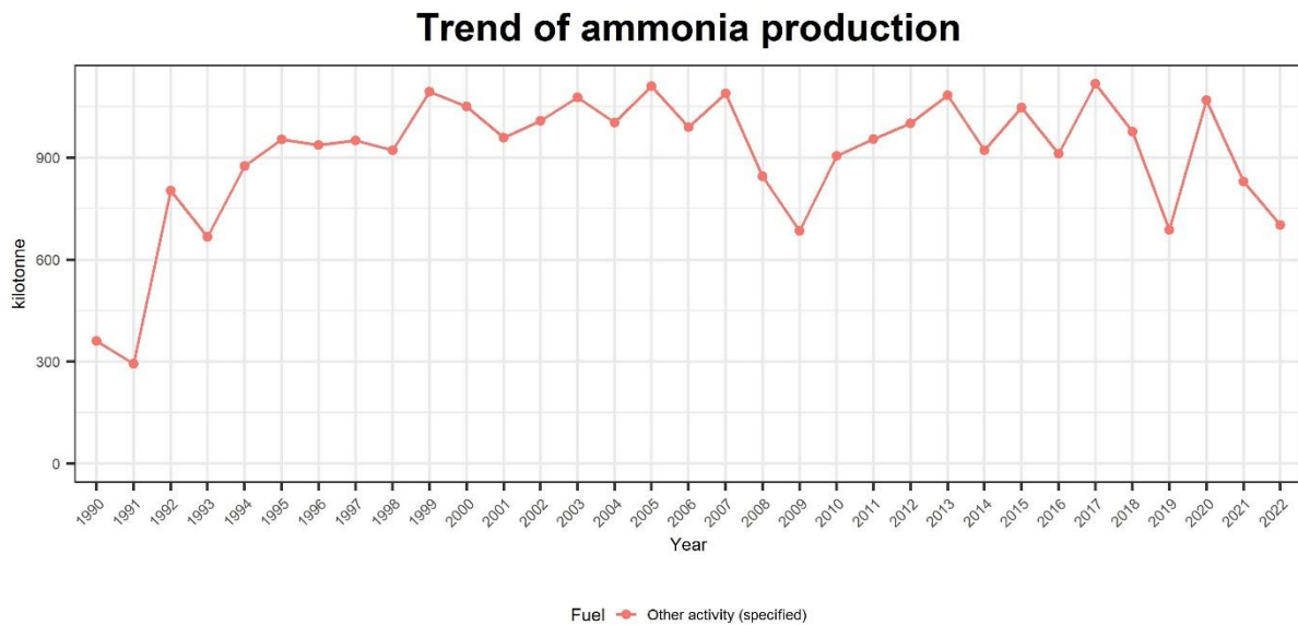
Figure 4 3 Trend of ammonia production.
