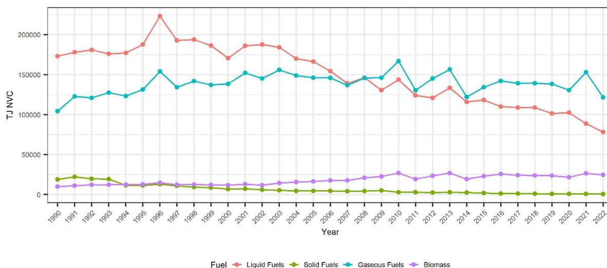
Figure 3 5 Trend of fuel consumption in the residential sector
