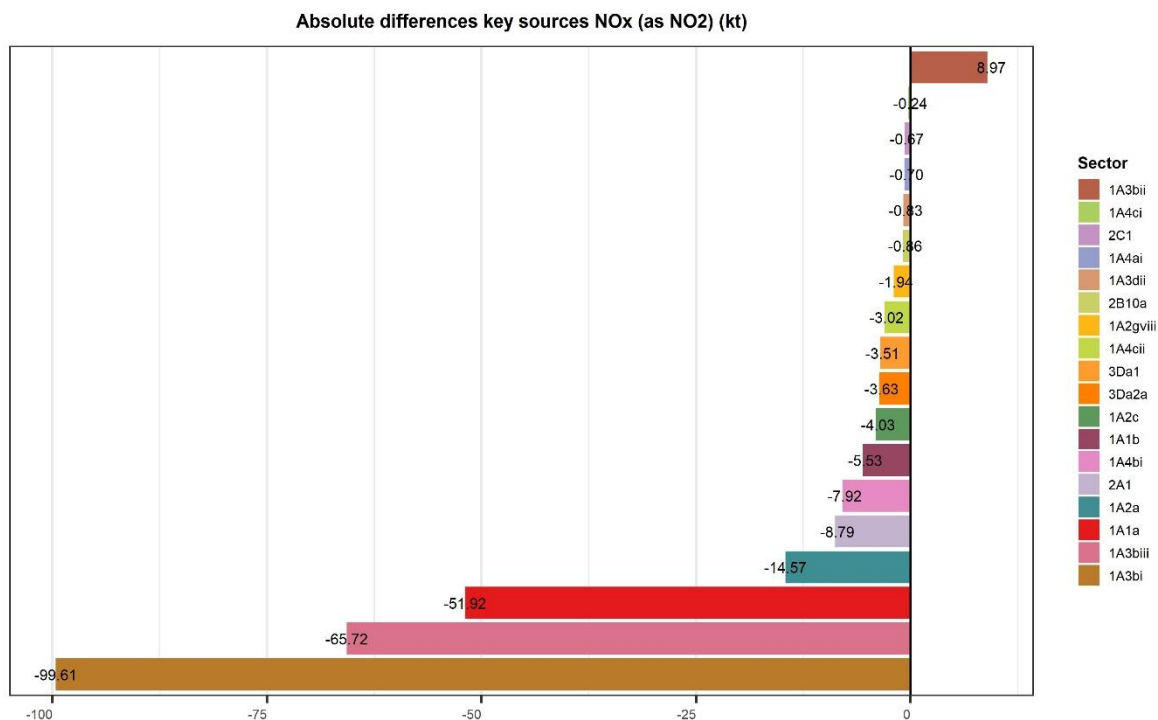
Figure 2 3 Absolute NO x emission differences from 1990 to 2022 for all key sectors
