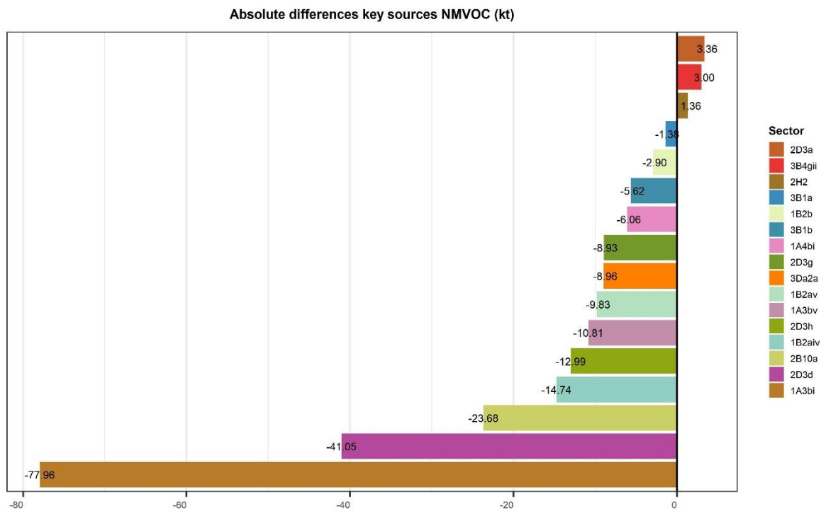
Figure 2 4 Trends in NMVOC emissions for the key sectors
