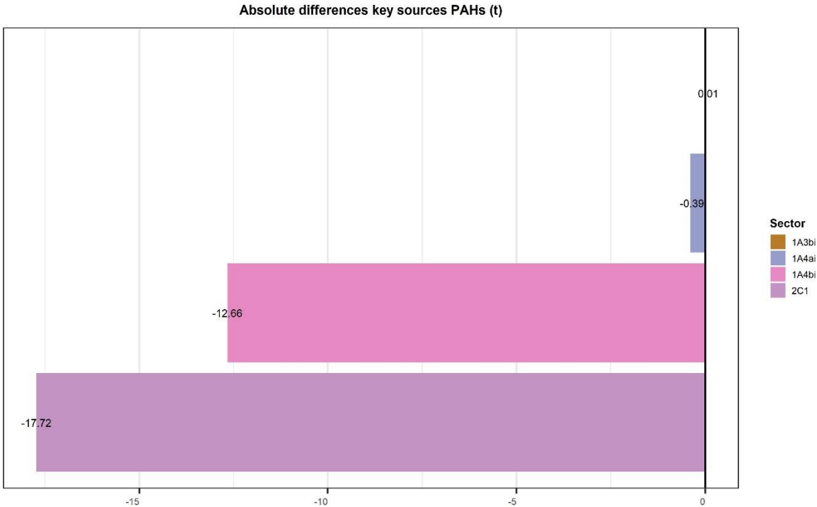
Figure 2 18 Trends in PAH emissions for the key sectors
