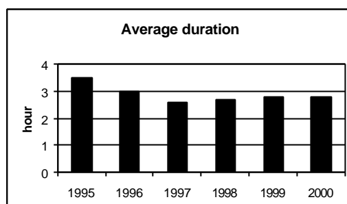
Figure 3.5.a. Average duration in hours of exceedances during the summer period (April-August, French and Italian data were not included in 1995 and 1996).
