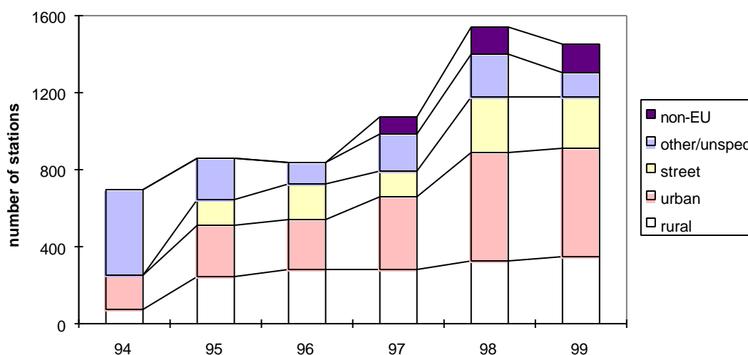
Figure 2.1. Number of stations reporting ozone data within the framework of the Ozone Directive. For stations in non-EU countries a station classification is known but not resolved in this figure for clarity.
