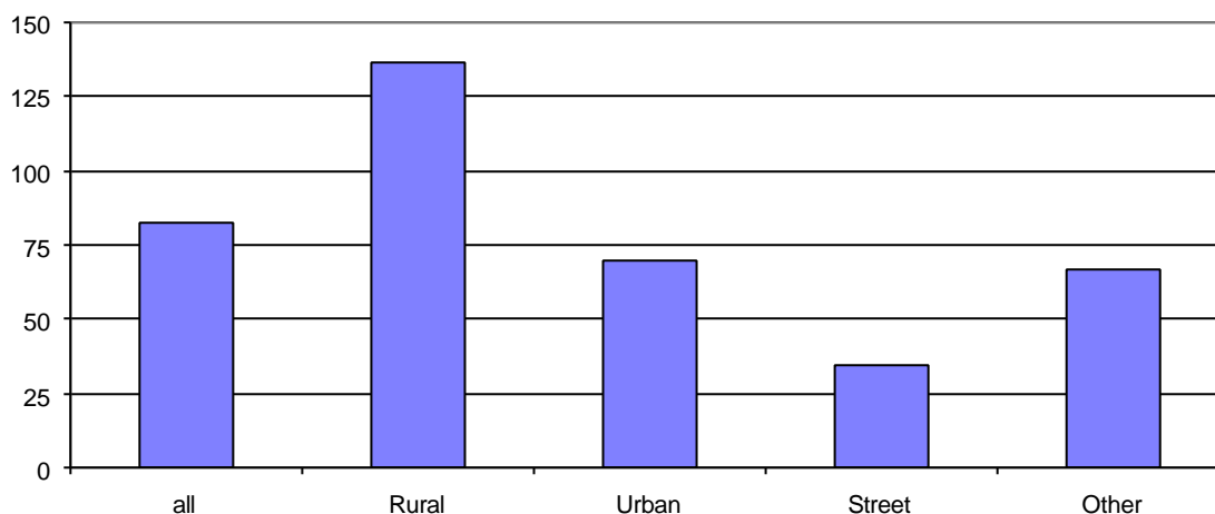
Figure 4.5. Occurrence of exceedance of the ozone daily threshold of 65 \mu\text{g}/\text{m}^3 as function of station type, averaged over all reporting countries; period 1 January - 31 December 1999
