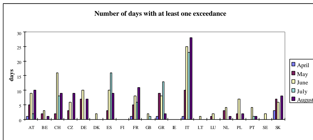
Figure 3.1. Number of days on which at least one exceedance of the threshold value for information of the public (1h ozone concentration > 180 \mu\text{g}/\text{m}^3 ) was observed per country 4 and per month during summer 2000. Finland and Ireland did not report exceedances. (Non-EU countries reporting no exceedances are not shown).
