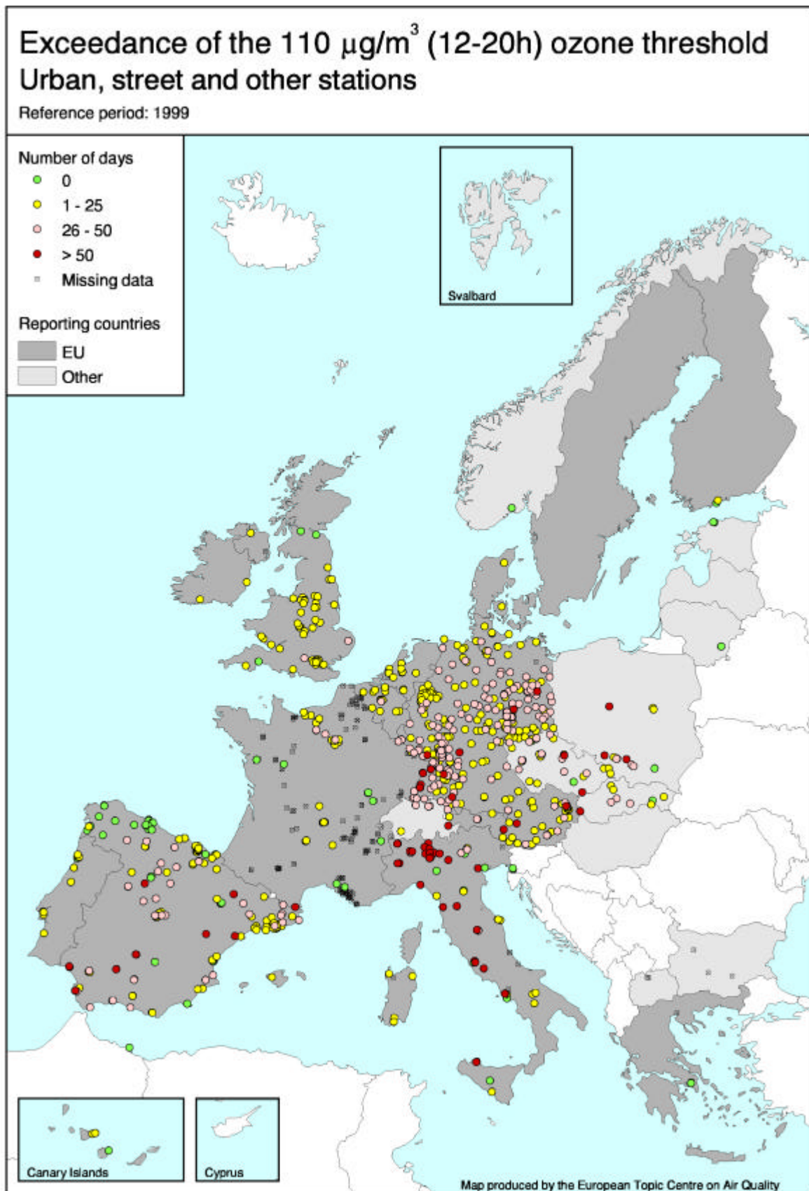
Map 4.4. Number of exceedances of the threshold value for protection of human health ( 110 \mu\text{g}/\text{m}^3 for 8h-values) observed at urban, street and other stations; 1 January - 31 December 1999; 8h- average values for the period 12.00-20.00.
