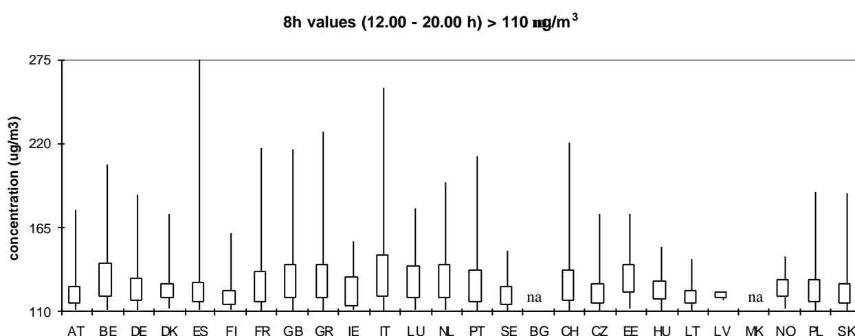
Figure 4.1. Frequency distribution of ozone concentrations (eight-hourly values; period 12.00-20.00;
