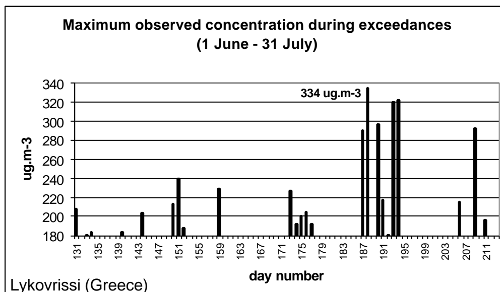
Figure 3.7. Example of frequent exceedances of the public information threshold value. Maximum observed 1h values ( \mu\text{g}/\text{m}^3 ) on the Lykovrissi monitoring station (Greece, 1 Jun –31 July 2000) on days when the concentration rose to at least 180 \mu\text{g}/\text{m}^3 (1h).
