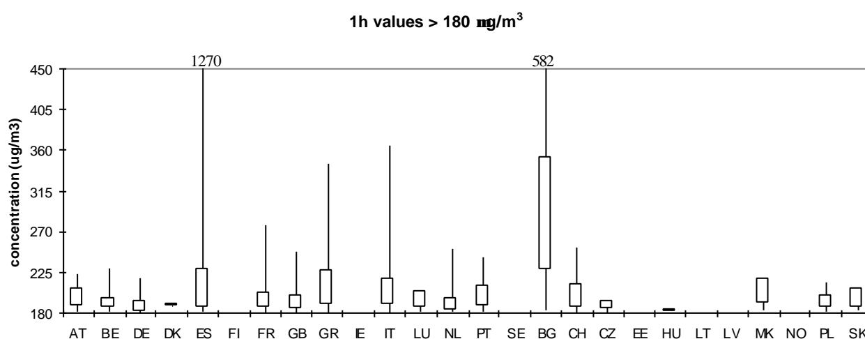
Figure 4.3. Frequency distribution of ozone concentrations (hourly values, 1 January - 31 December 1999) in excess of the 180 \mu\text{g}/\text{m}^3 threshold for hourly values. Frequency distributions are presented as Box-Jenkins plots indicating the minimum, the 25-percentile, the 75-percentile and the maximum value (in \mu\text{g}/\text{m}^3 ). The maximum concentrations measured in Spain ( 1270 \mu\text{g}/\text{m}^3 ) is possibly a measuring artefact. In Finland, Ireland, Sweden, Estonia, Lithuania, Latvia and Norway no exceedances of this threshold have been reported.
