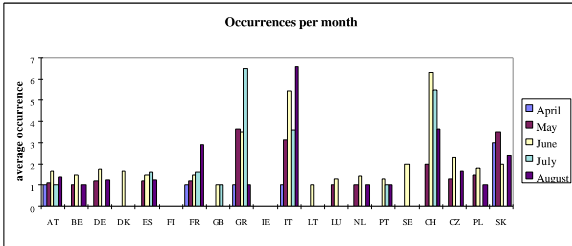
Figure 3.2. Occurrence of exceedances of the threshold value for information of the public (1h ozone concentration > 180 \mu\text{g}/\text{m}^3 ) per country on a month by month basis during summer 2000. Finland, and Ireland did not report exceedances. (Non-EU countries reporting no exceedances are not shown).
