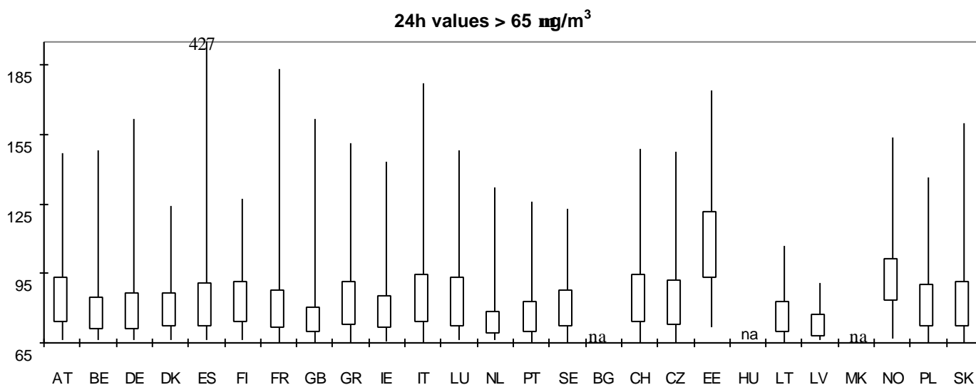
Figure 4.6. Frequency distribution of ozone concentrations (24h values; 1 January - 31 December 1999) in excess of the 65 \mu\text{g}/\text{m}^3 -threshold for daily values. Frequency distributions are presented as Box-Jenkins plots indicating minimum, 25-percentile, 75-percentile and
