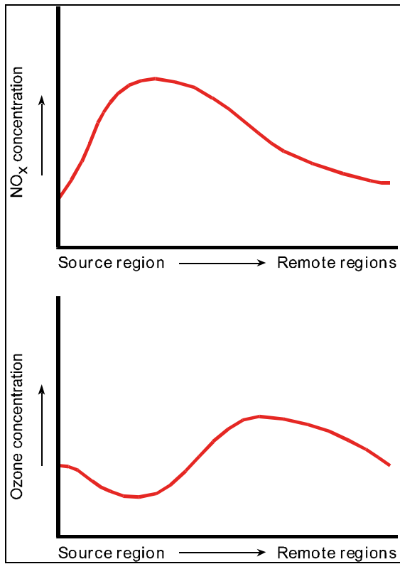
Figure 1.7 Schematic view of the development of \text{NO}_x and ozone levels in air passing over a source region
