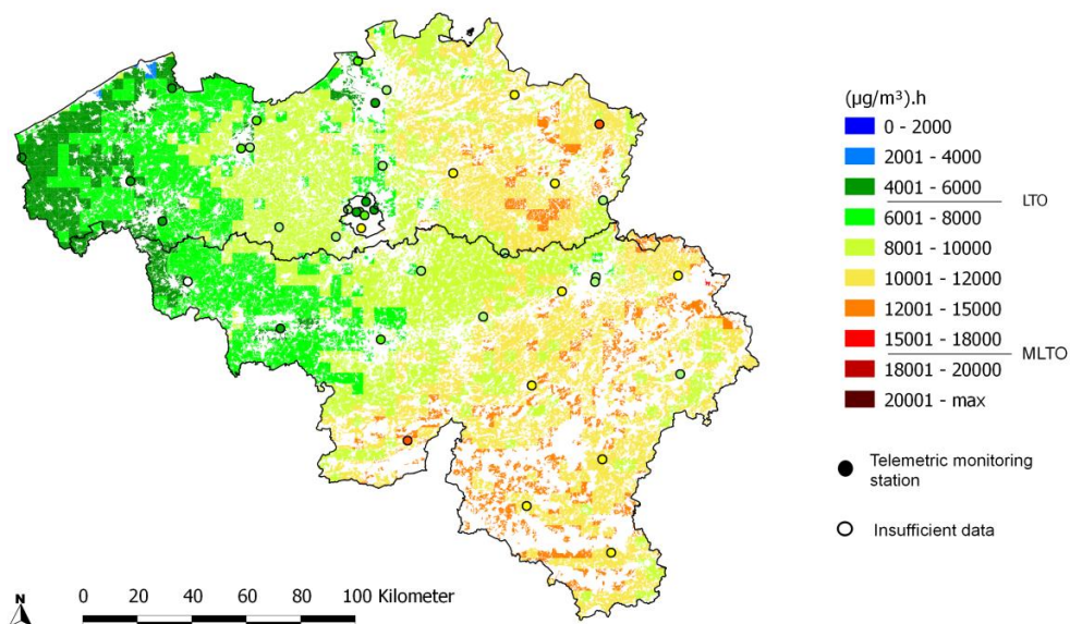
AOT40 vegetation (Belgium, 2008 - 2012)
