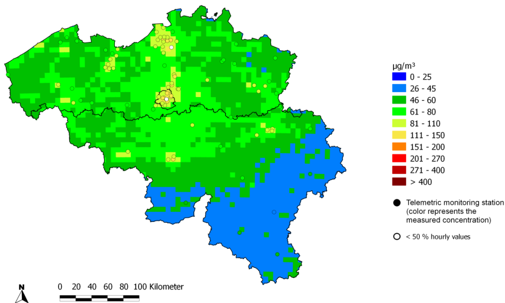
19th highest NO 2 concentration (Belgium, 2012)
