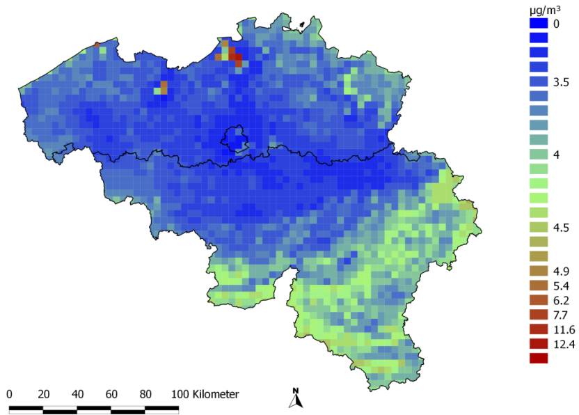
O 3 Annual mean absolute error (Belgium, 2012)
