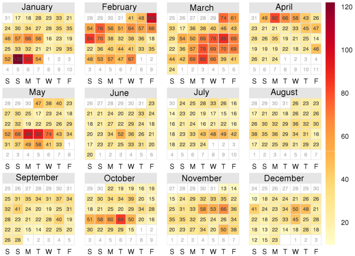
Mean daily PM 10 concentrations in 2012
