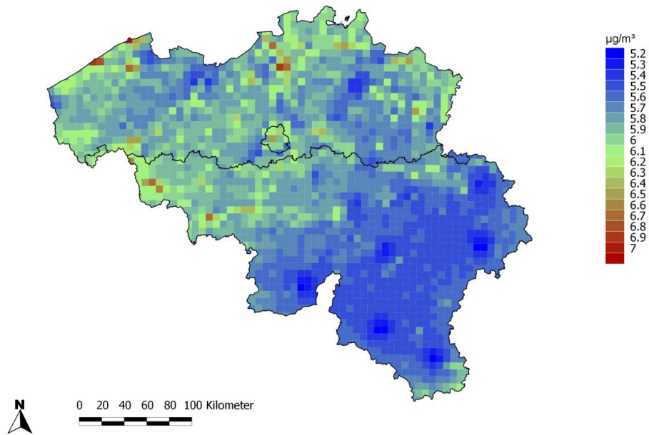
Error on NO 2 annual mean (Belgium, 2012)
